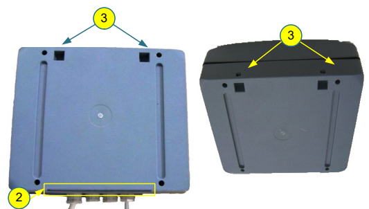
Figure 5-18: Control Module's Mounting Interface
