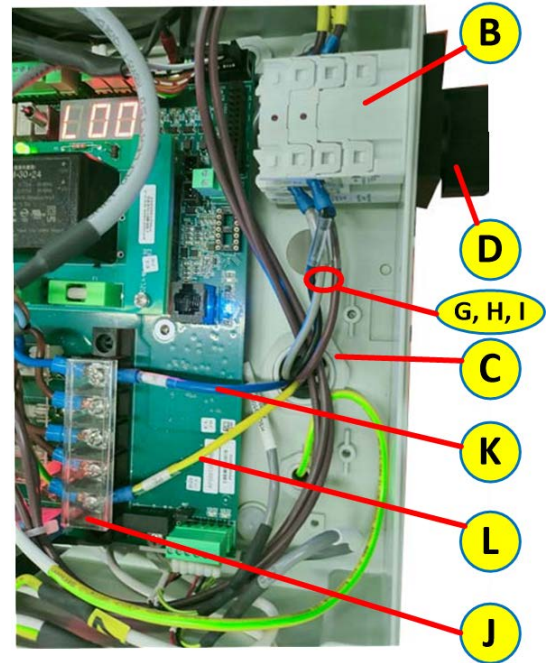
Figure 5-39: Power cable connections to connection box
