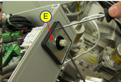
Figure 5-41: Replacing the Power Cable 2
