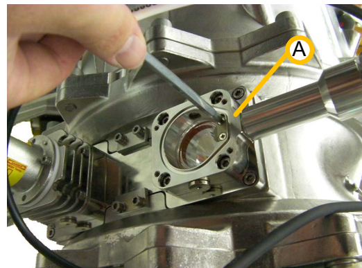
Figure 10-20: (Generic) Cleaning the UV Intensity Sensor's Mirror
