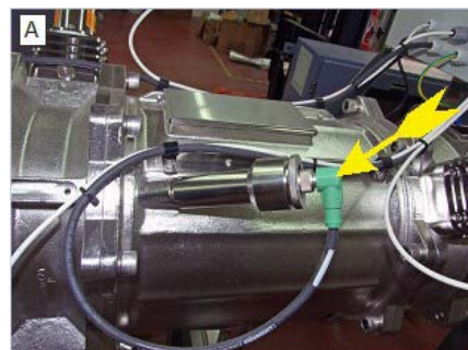
Figure 10-27: Removing a Sensor A (Generic View)
