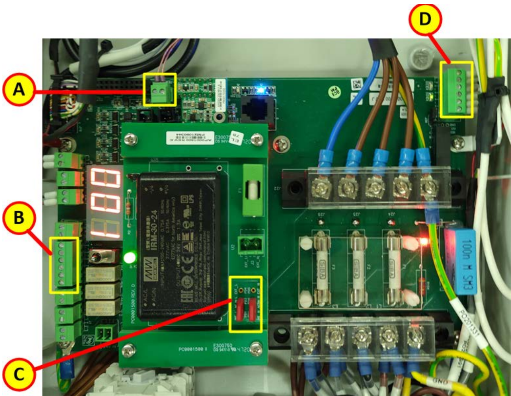
Figure 5-32: Connection Box LM Card 1300+1500 (for RZ system without cleaner)
