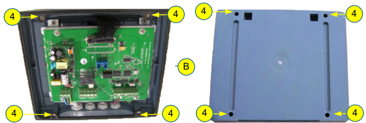
Figure 5-24: Control Module's Circuit Board
