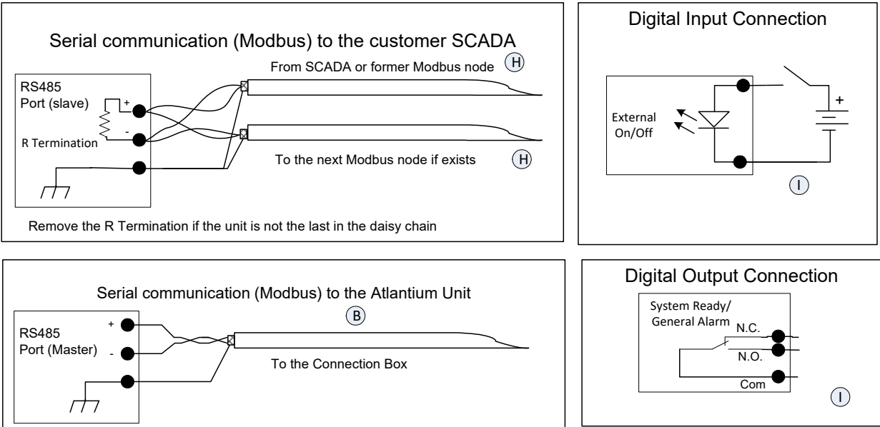
Figure 5-23: Control Module Terminal Connectors Wiring Drawings
