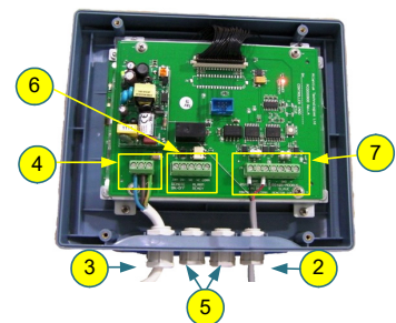
Figure 5-20: Control Module's Circuit Board
