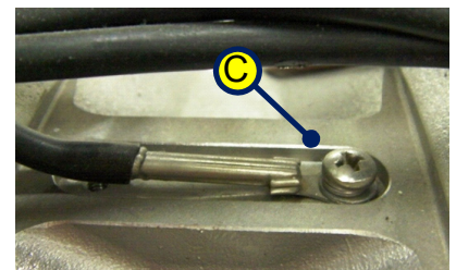
Figure 10-40: Location of the Temperature Sensor on the Atlantium Unit
