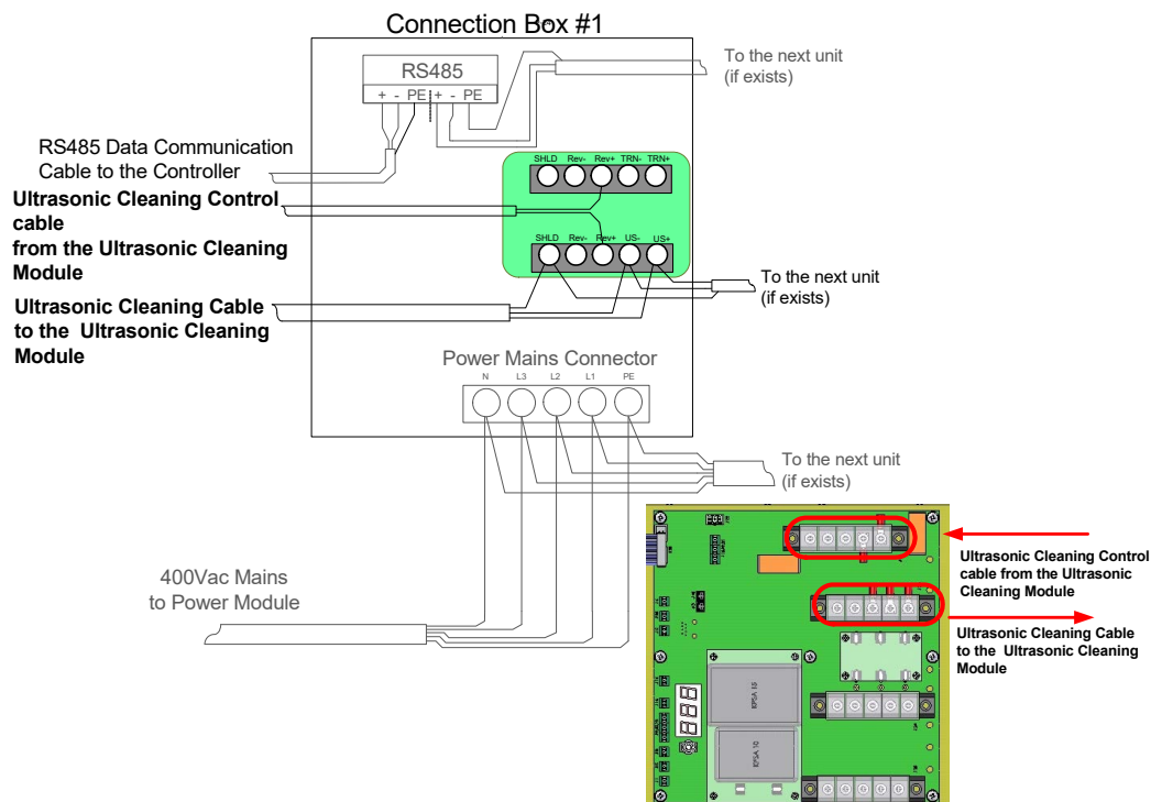
Figure 5-33: Cabling Schematic Diagram
