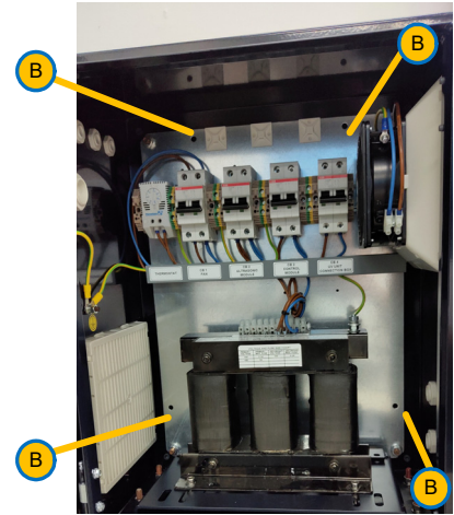
Figure 5-25: Power Module - Mounting Holes
