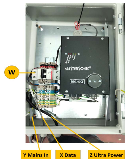
Figure 5-35: Ultrasonic Cleaner Module - Inside View
