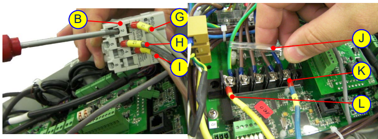
Figure 5-44: Replacing the Power Cable 5
