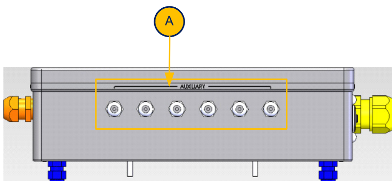
Figure 5-30: Connection box with cable insertion holes (A)
