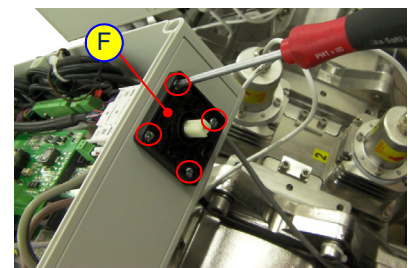
Figure 5-42: Replacing the Power Cable 3
