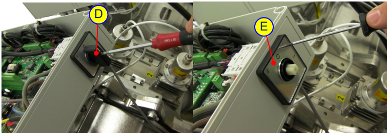
Figure 5-40: Replacing the Power Cable 1
