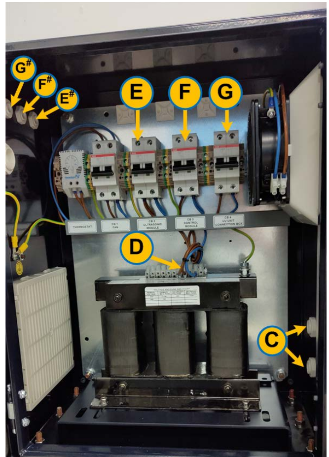
Figure 5-37: Power Module - connections
