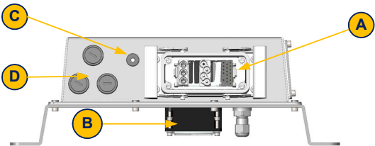
Figure 5-28: Ballast Module C-Waterproof Box (bottom view)
