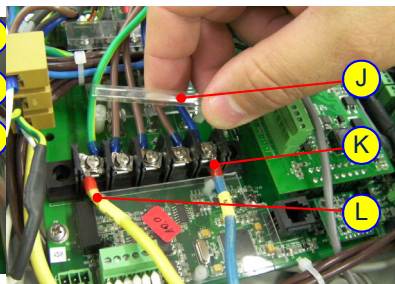
Figure 5-44: Replacing the Power Cable 5
