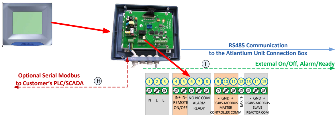
Figure 5-22: Control Module Terminal Connectors Schematic Drawing
