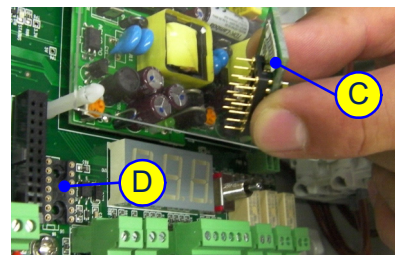
Figure 10-41: Replacing the Temperature Sensor Card (Generic)
