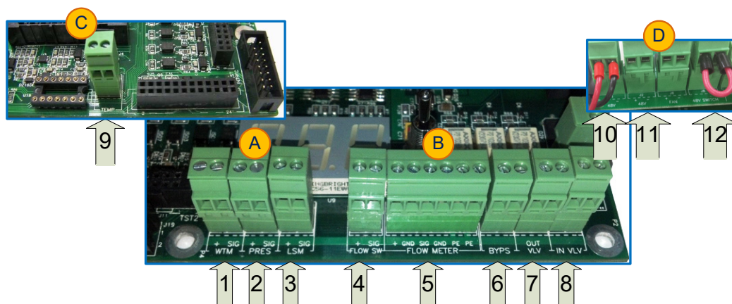
Figure 5-38: Connectors on Connection Box Card I300+I400
