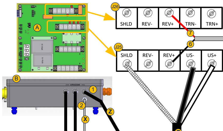
Figure 5-34: Ultrasonic Cleaner Cable Connections in the Connection Box
