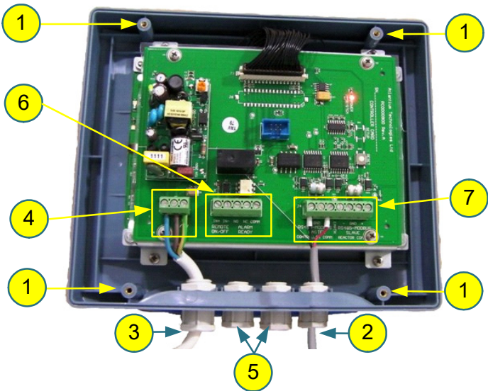
Figure 5-15: Control Module Interior
