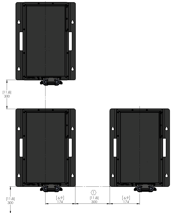
Figure 5-27: Multiple Ballast Module C Installation Diagram
